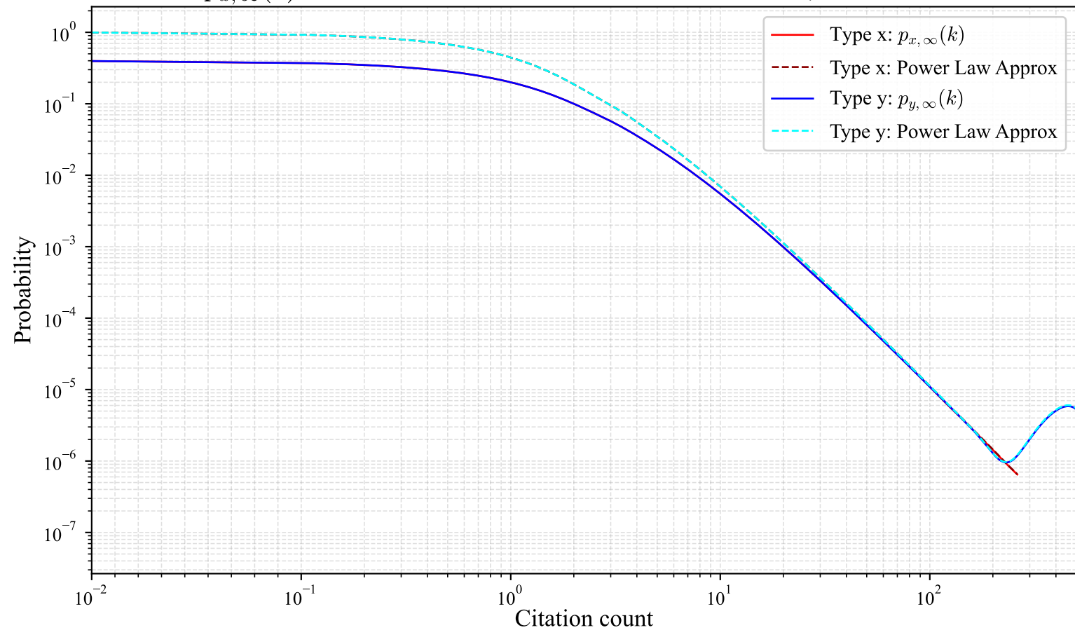
p_{x,\infty}(k) vs Power Law for Citation Distribution in 28,005 Network
